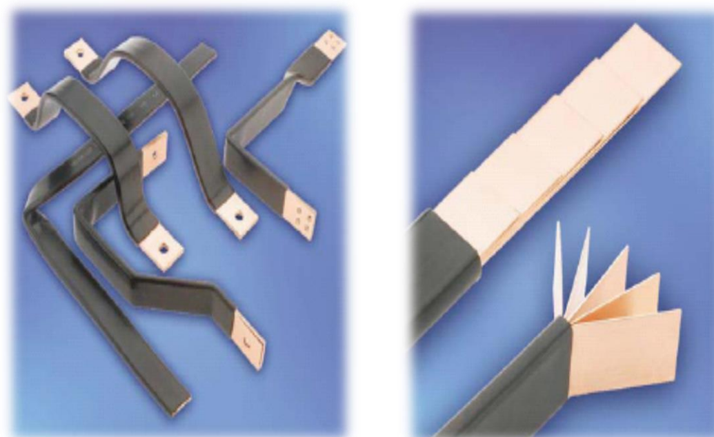
Insulated flexible lamellas and bars
