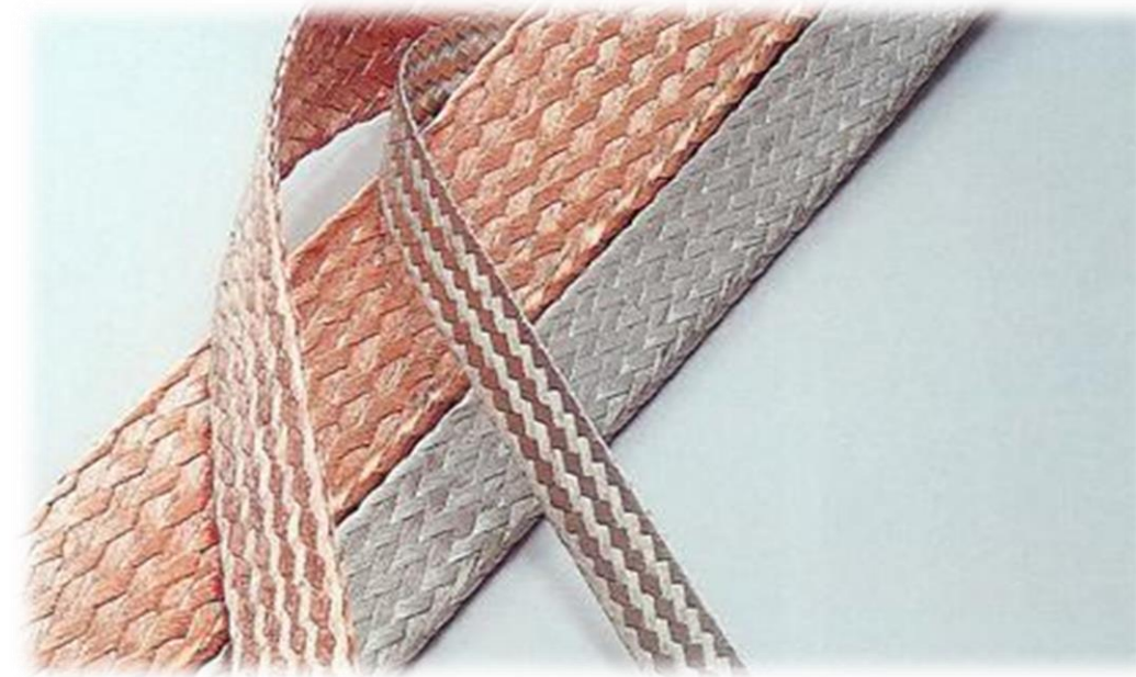
Flat braided 0,16mm 2 - 400mm 2
